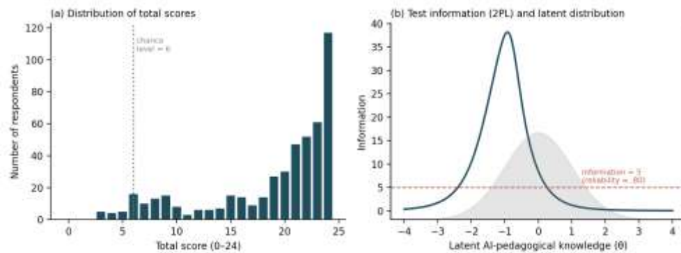
Figure 1. (a) Distribution of Part B total scores ( N = 484 ). (b) Test information function based on 2PL parameters, with the standard normal latent distribution shaded.
